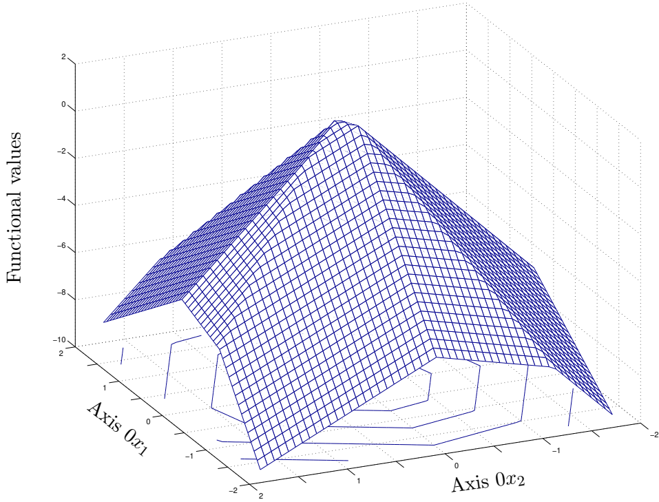
Figure 9: The graph of the recognizing functional of the tolerable solution set to the system (10).
