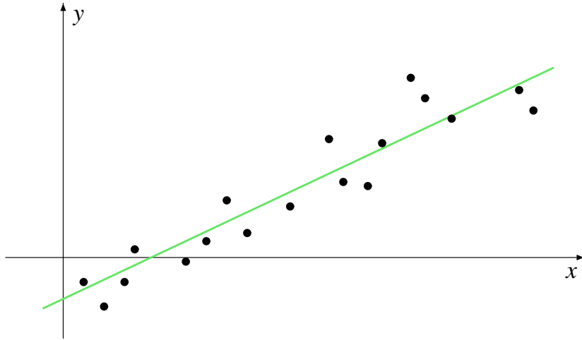
Figure 1: Illustration of the data fitting problem
