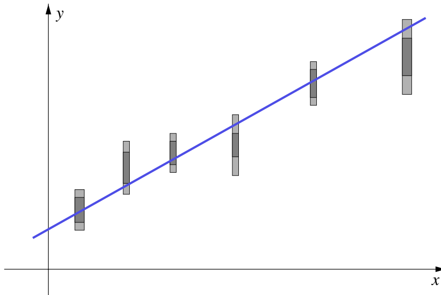
Figure 10: Expanding the data uncertainty boxes along the output variables leads to the strong compatibility.
