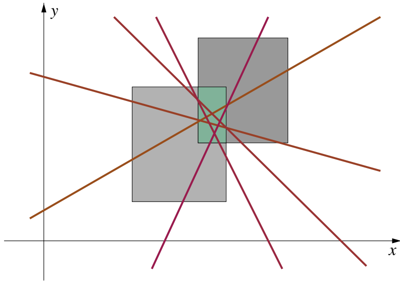
Figure 11: The intersection of boxes may result in total indeterminacy of the angular coefficient of the line passing through the boxes in the sense of “weak compatibility”.
