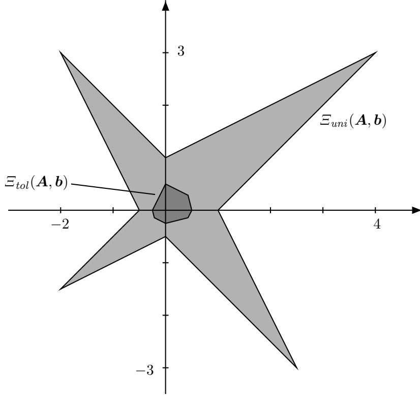
Figure 6: United solution set and tolerable solution set for the interval system of linear equations (10)
