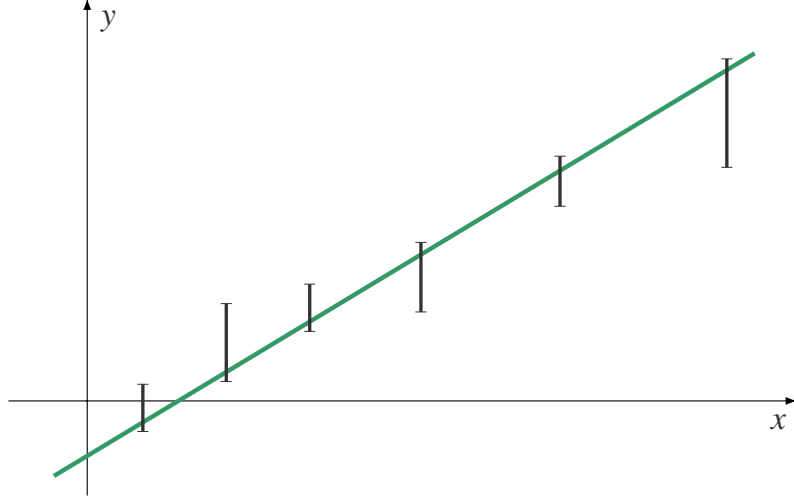
Figure 2: Illustration of the compatibility between parameters of a linear model and interval measurement data for exact values of the independent variable.
