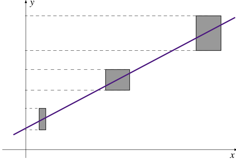
Figure 4: Illustration of the strong compatibility between parameters of a linear model and interval measurement data.
