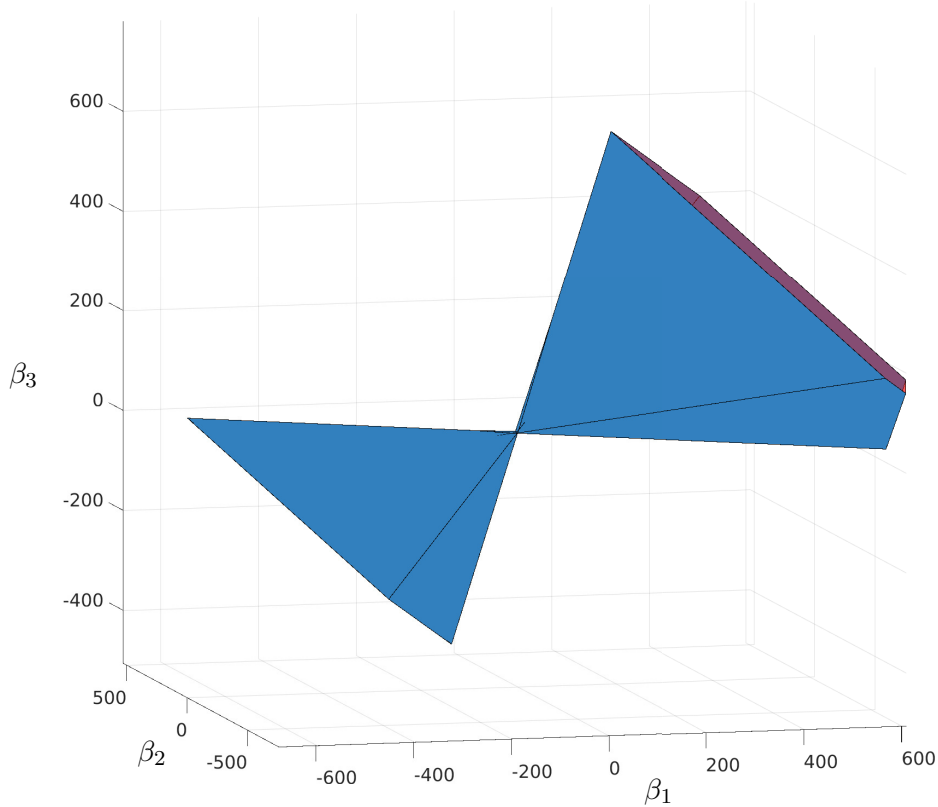
Figure 13: The unbounded united solution set to the interval linear system (15).
