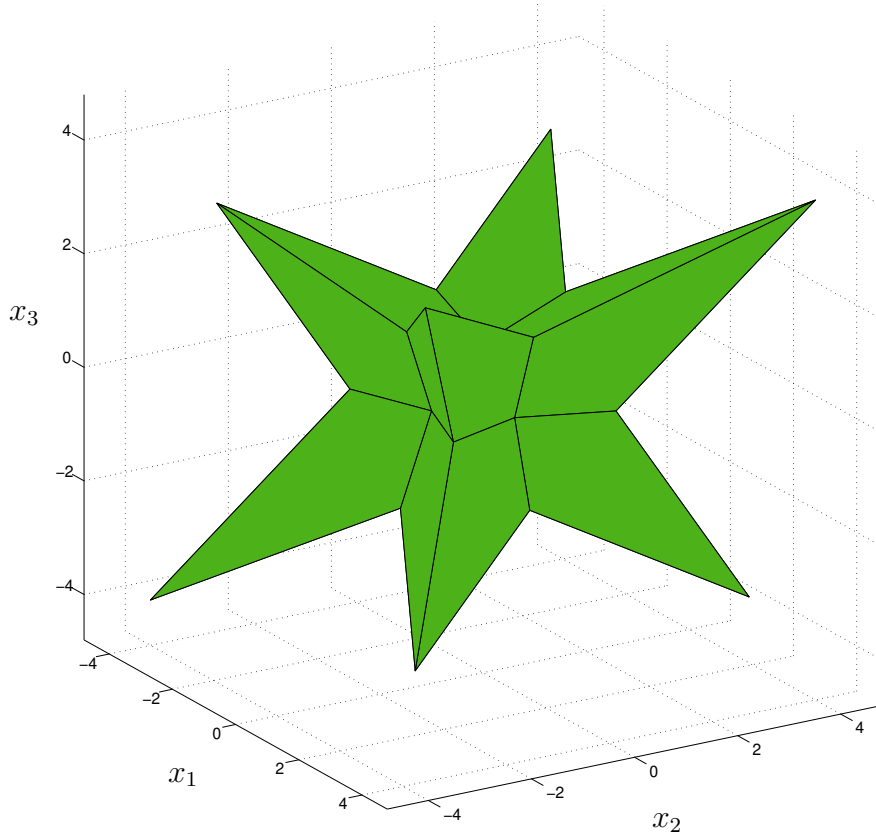
Figure 7: United solution set for the interval system (11).
