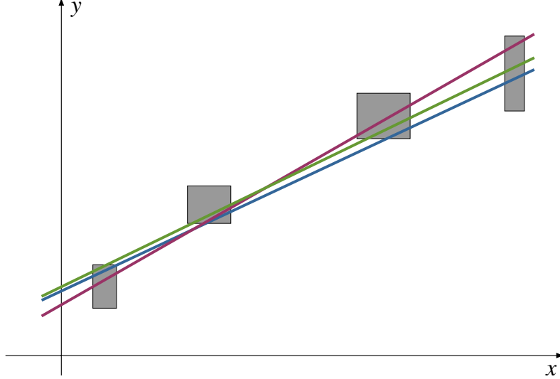
Figure 3: Illustration of compatibility between parameters of a linear model and interval measurement data in the general case.
