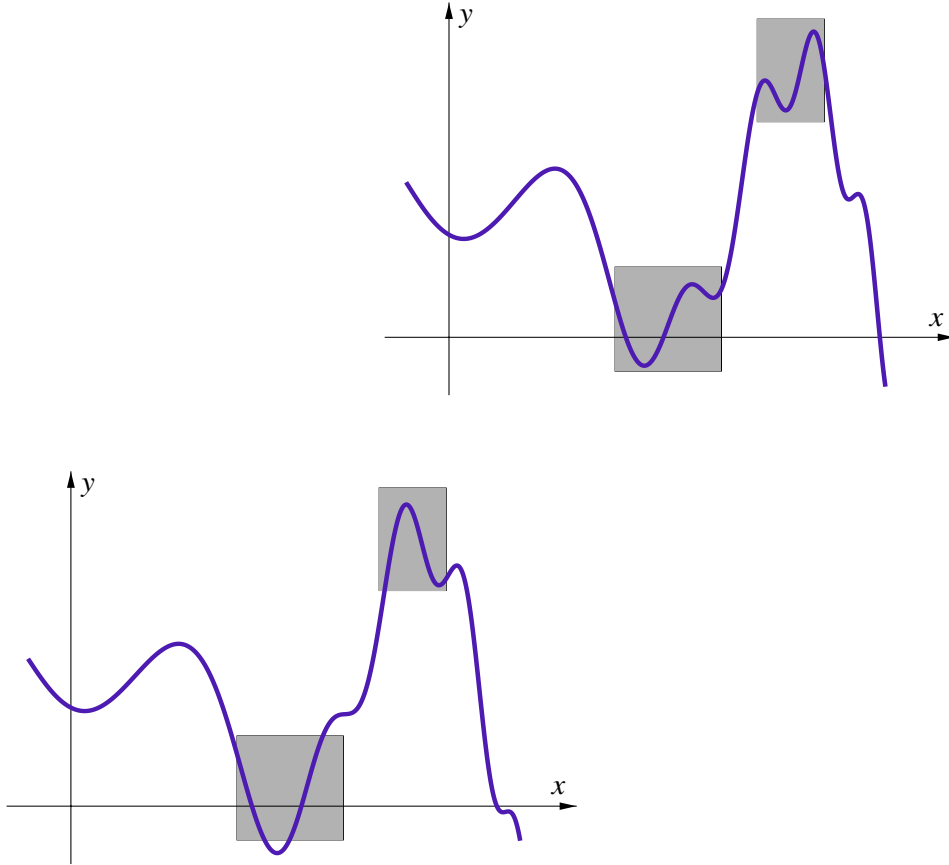
Figure 5: Illustration of the weak (below) and strong (above) compatibility between parameters of a nonlinear model and interval measurement data.
