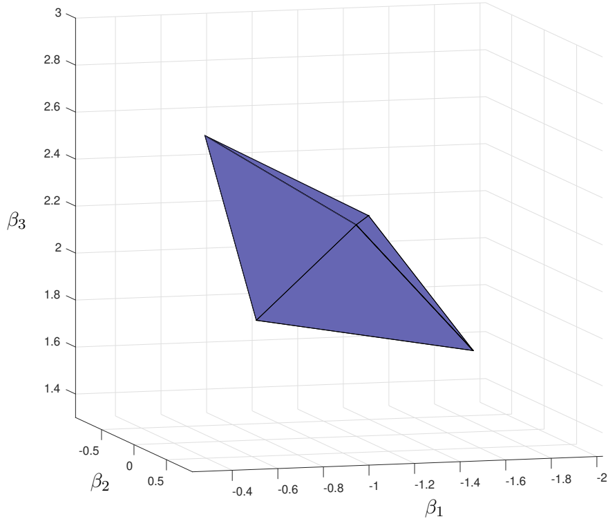
Figure 14: The tolerable solution set to the interval linear system (15).
