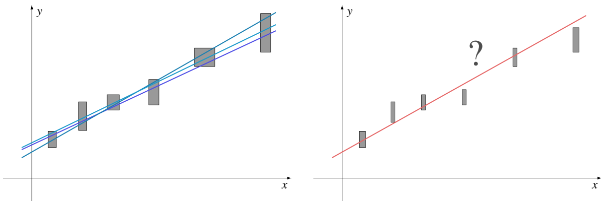
Figure 12: Wide uncertainty boxes enable us to construct many models compatible with the data. For narrow uncertainty boxes, a model compatible with the data may not exist.
