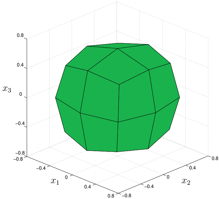
Figure 8: Tolerable solution set for the interval system (11).
